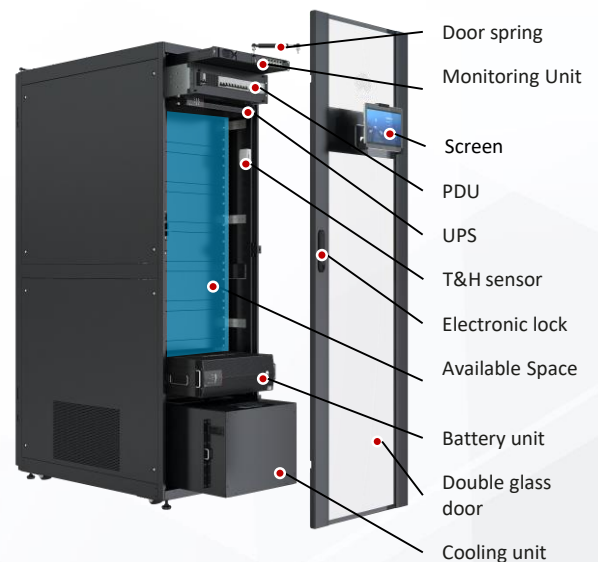
FusionModule500 Architecture
